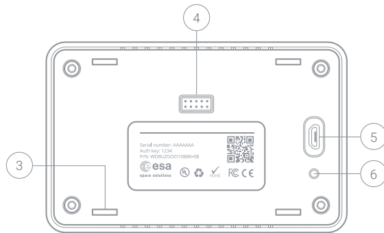
Sensing unit back side
